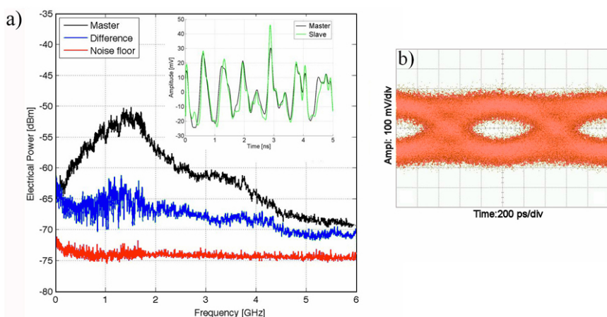
Figure 3. (a) Power spectrum of the emitter laser (black line), difference between emitter and receiver power spectra under synchronized conditions (blue line) and noise floor (red line). (b) Recovered eye diagram of a 1Gb/s non-return to zero random sequence. mV/div: Millivolt per division. ps/div: Picosecond per division.
