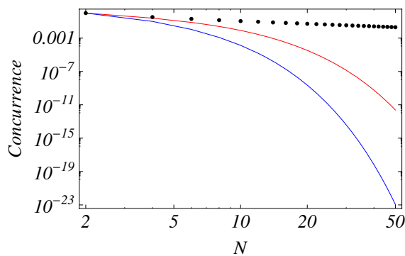
Fig. 2 (online colour at: www.fp-journal.org ) Two-spin concurrence as a function of the system size N for the XXX model (dots) and for the XY model (continuous lines). In this latter case, we considered two different anisotropy parameters: the red line represents \gamma = 0.5 , and the blue line corresponds to \gamma = 0.8 .
