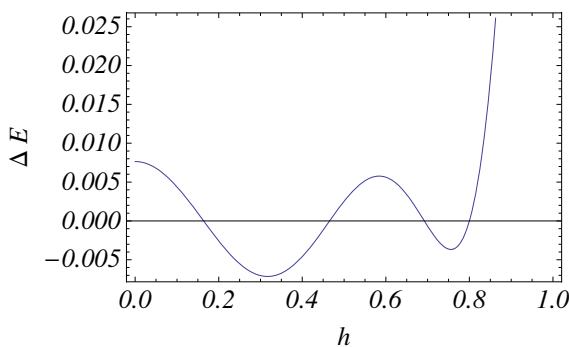
Fig. 1 (online colour at: www.fp-journal.org ) Difference of energy between the lowest odd and even eigenvalues of H as a function of the transverse field for a 8-spin chain. Given the anisotropy amplitude \gamma = 0.6 , the factorizing field is h_F = 0.8 . As predicted, we observe N/2 level crossing point, the last of them being h_F .
