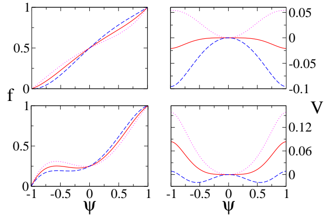
FIG. 1: Flipping probability f (left boxes) and its associated potential V (right boxes) vs local field \psi . Curves correspond to coefficient values a = -0.3 (dotted), a = 0 (solid), a = 0.3 (dashed), for b = -0.25 (top) and b = 1.0 (bottom). For both values of b , a single-well and double-well potentials are obtained for a < 0 and a > 0 respectively.
