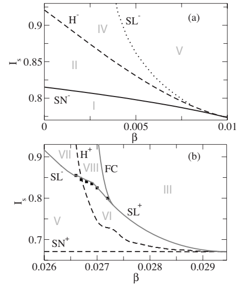
FIG. 2. Zoom of Fig. 1 near TB_1 (a) and TB_2 (b). Lines have been determined using the method explained in Sec. III A with the exception of the SL line in (b). In that case, the filled squares display the location of the SL obtained from numerical integration of Eq. (1), while the gray line through these points is only to guide the eye. \theta = 1.23 .
