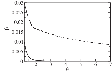
FIG. 9. Location (\theta_{TB}, \beta_{TB}) of the two TB points as the detuning is increased. The solid and dashed lines correspond to the TB_1 and TB_2 points, respectively.
