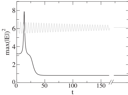
FIG. 8. The conditional excitability regime is illustrated for \beta = 0.0272 and I_s = 0.8 . The solid line (excitable trajectory) corresponds to time evolution of the maximum of the peak after a localized perturbation of the homogeneous state that brings the system beyond the excitability threshold but outside the basin of attraction of the upper branch DS. The gray line corresponds to a more strongly localized perturbation that brings the system inside the boundary of attraction of the upper branch DS.
