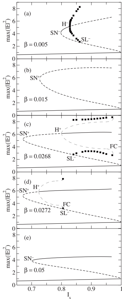
FIG. 4. Bifurcation diagrams showing the maximum intensity of the DS as a function of the background intensity I_s , for \beta = (a) 0.005, (b) 0.015, (c) 0.0268, (d) 0.0272, and (e) 0.05. The lowest solid line represents the stable homogeneous solution. The lowest dashed line shows the maximum intensity of the unstable middle branch DS. Above that line, the upper branch DS is shown, where the solid line stands for the stable DS and the dashed line for the unstable DS. In (a), (c), and (d) the system exhibits stable oscillatory behavior (see text). In these cases, the maximum and minimum intensity of the oscillating DS are depicted as filled squares. The gray dashed line, representing the unstable limit cycle, is only a guiding line for the eye. When the limit cycle touches the middle branch DS, a saddle-loop bifurcation occurs. \theta=1.23 .
