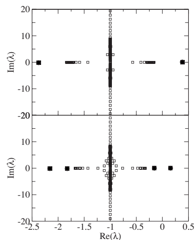
FIG. 7. Spectrum of the middle branch DS at the saddle-loop bifurcation for (a) \beta=0.0268 and I_s=0.84 and (b) \beta=0.0294 and I_s=0.671 . The filled black circles are the eigenvalues corresponding to the modes with a localized spatial profile. \theta=1.23 .
