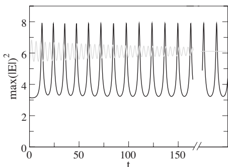
FIG. 5. Dynamical evolution of the system in the tristable regime, where the spatially homogeneous fundamental branch (not shown), stable oscillatory DS regime (solid line), and stable focus (gray line) coexists.
