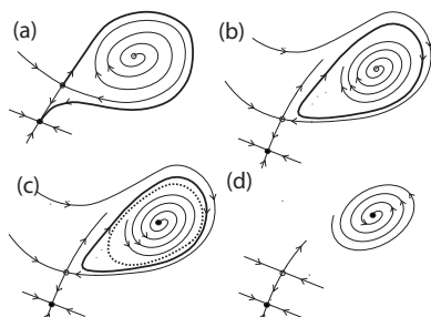
FIG. 6. Qualitative sketch of the phase space at I_s \approx 0.9 and \theta = 1.23 for increasing values of \beta , corresponding to a horizontal cut of Fig. 2(b). As \beta increases from (a) to (d), one starts with an excitable DS (region V), going through a region of bistability between a stable limit cycle and the stable homogeneous solution (region VII), followed by a coexistence of stable and oscillatory DSs (region VIII), and finally a stable DS (region III).
