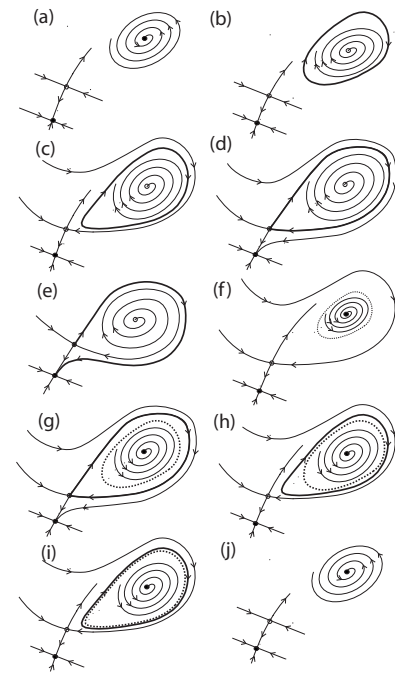
FIG. 3. Qualitative evolution of the phase space at I_s \approx 0.8 and \theta = 1.23 for increasing values of \beta , corresponding to the different dynamical behavior in a horizontal cut of Fig. 1. From (a) to (j), one goes from a stable DS (region II) to an oscillating DS (region IV), followed by an excitable DS (region V), a conditional excitable DS (region VI), a coexistence of stable and oscillatory DSs (region VIII), and finally a stable DS (region III).
